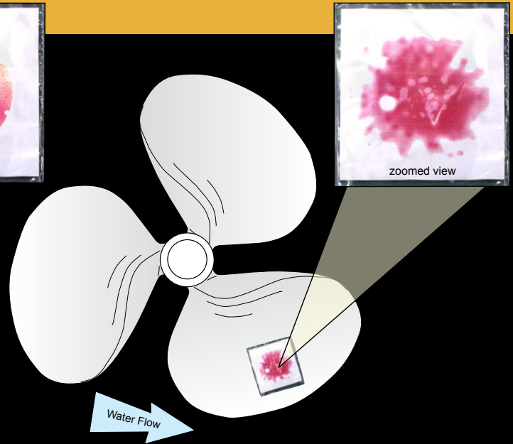
Encased Fujifilm Prescale® film used in a propeller test
