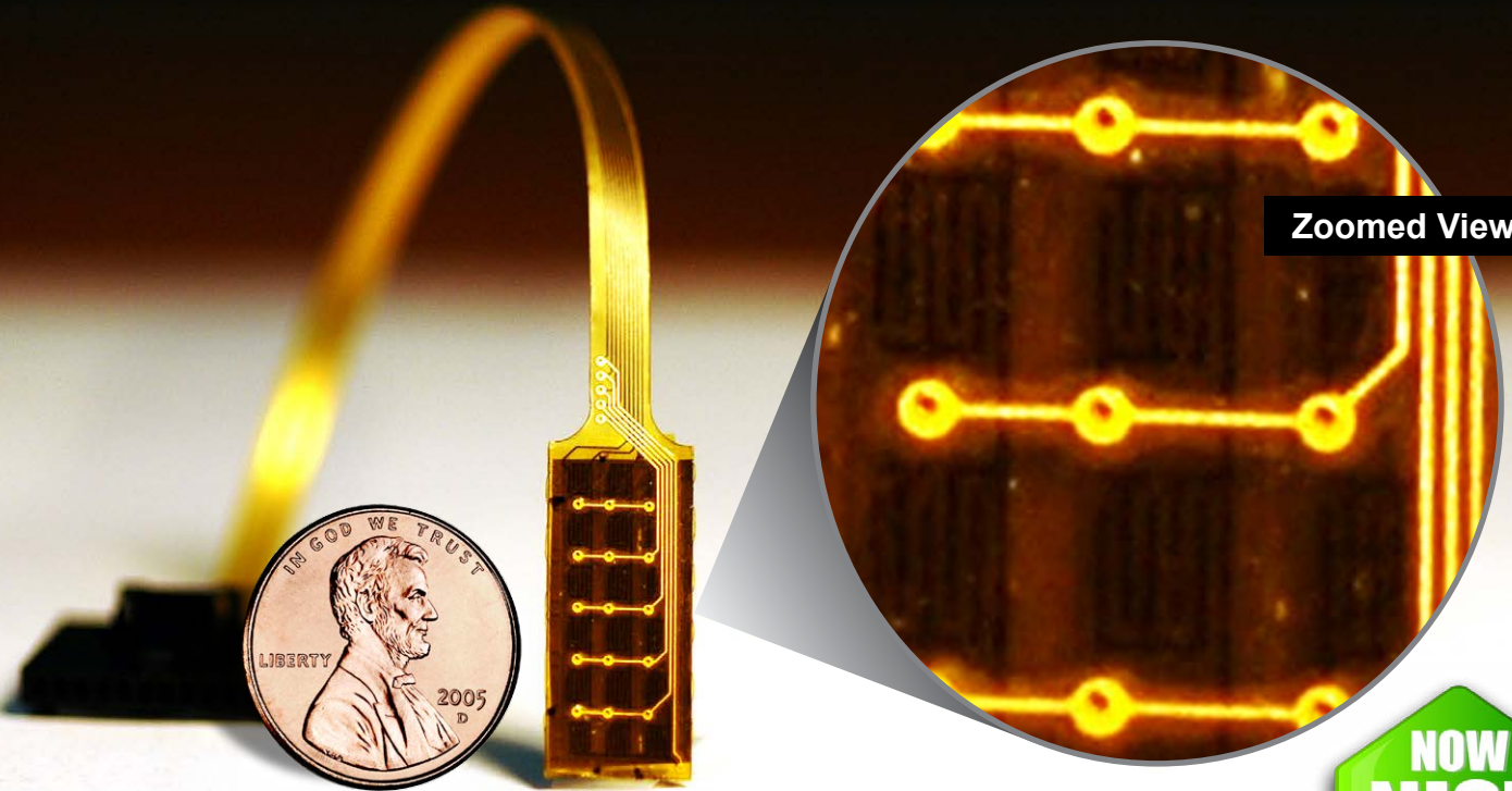
Tactilus T-Series Sensor with 18 Sensing Points Spaced 2 mm Apart
