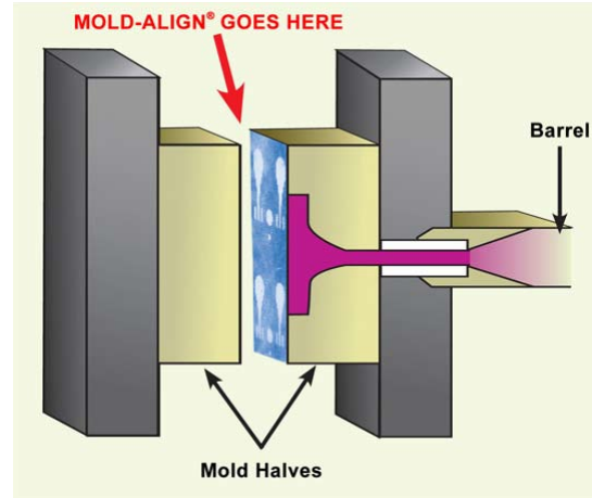
Pressure Film ensures precise mating between mold halves.
