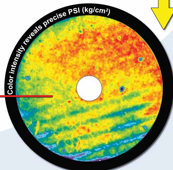
Fuji Prescale® film AFTER Topaq® Analysis
