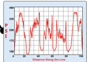
Pressure Profile
