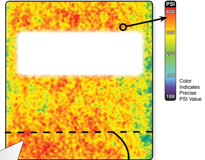
Pressure Profile
