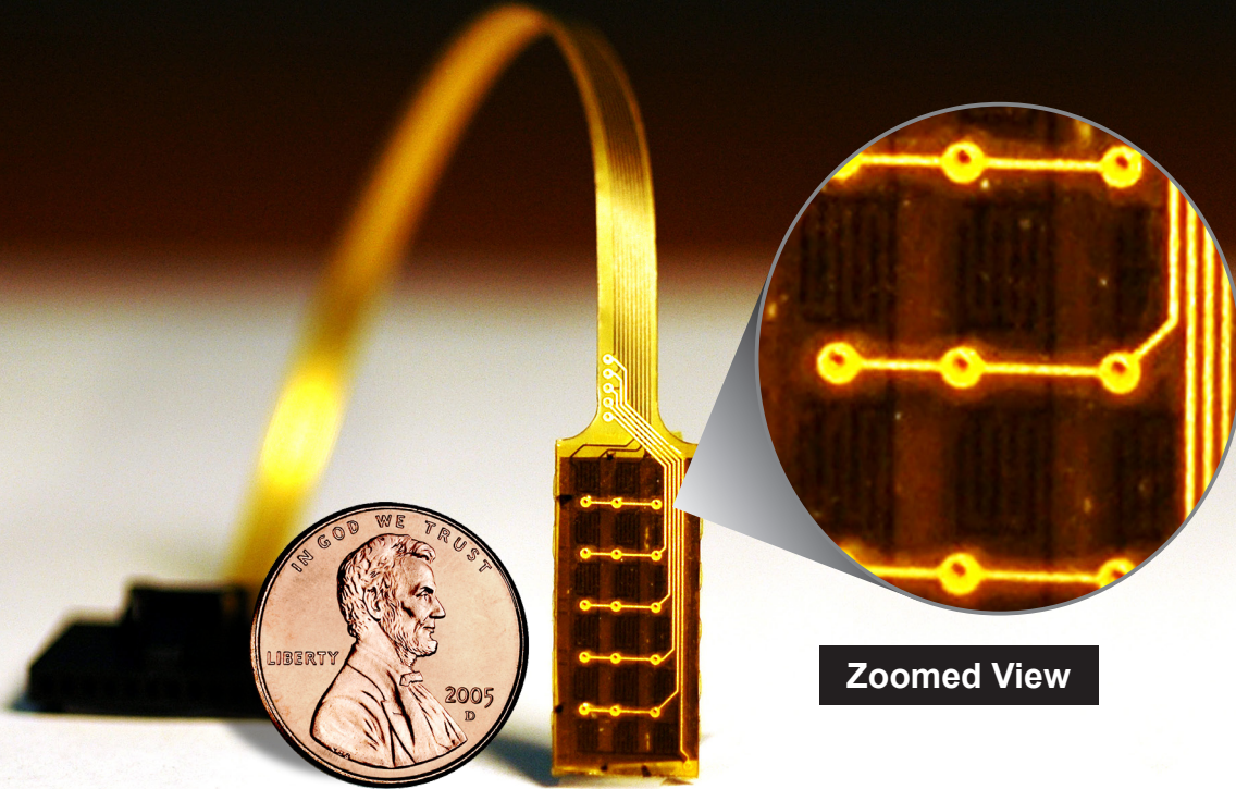
Tactilus T-Series Sensor with 18 Sensing Points Spaced 2.5 mm Apart
