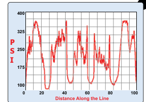
Pressure Profile
