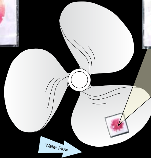
Encased Pressure x ® film used in a propellor test
