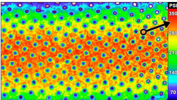
Nip Pressure Profile Film from Sensor Products Inc.
