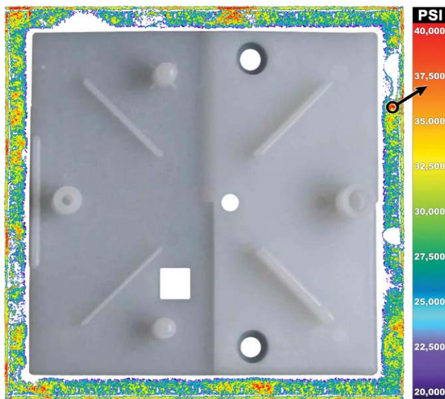
Pressurex distribution along the parting line of a mold
